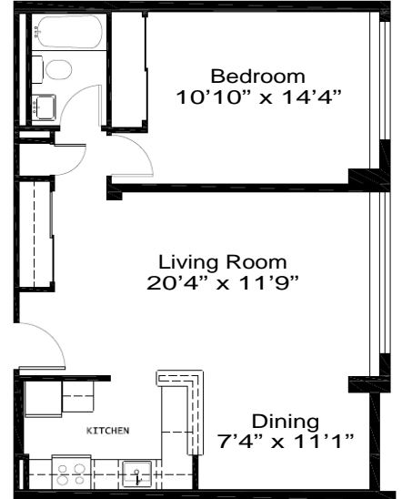
ONE BEDROOM TIER 21
