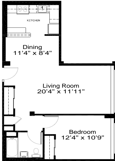
ONE BEDROOM - H.C. TIER 22 - FIRST THRU 6TH FLOORS
