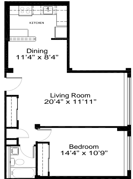
ONE BEDROOM TIER 22 - 7TH AND 8TH FLOORS
