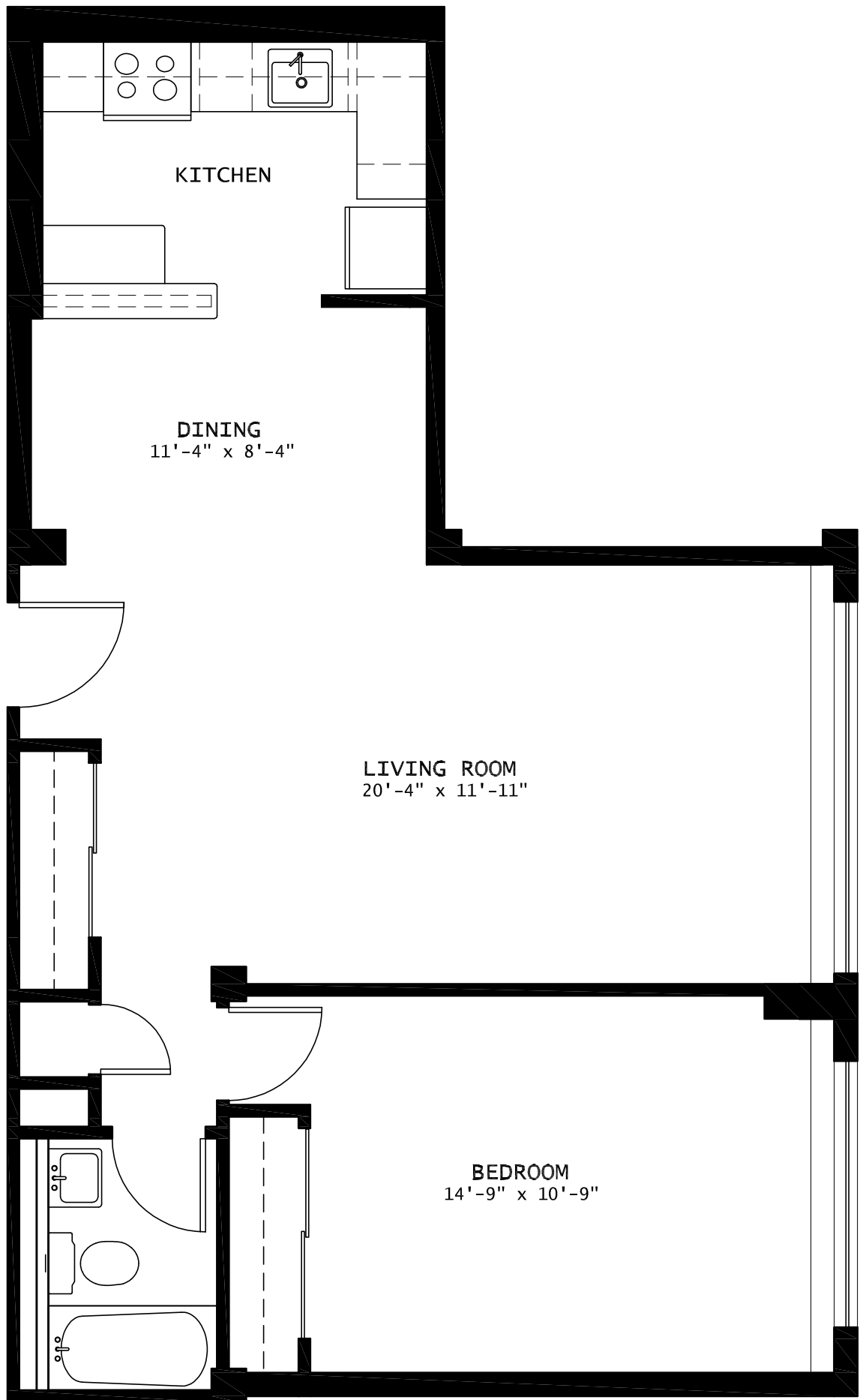
ONE BEDROOM TIER 22 - 7TH AND 8TH FLOORS
